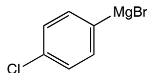
H51163 4-Chlorophenylmagnesium bromide, 1M in 2-MeTHF CAS 873-77-8
